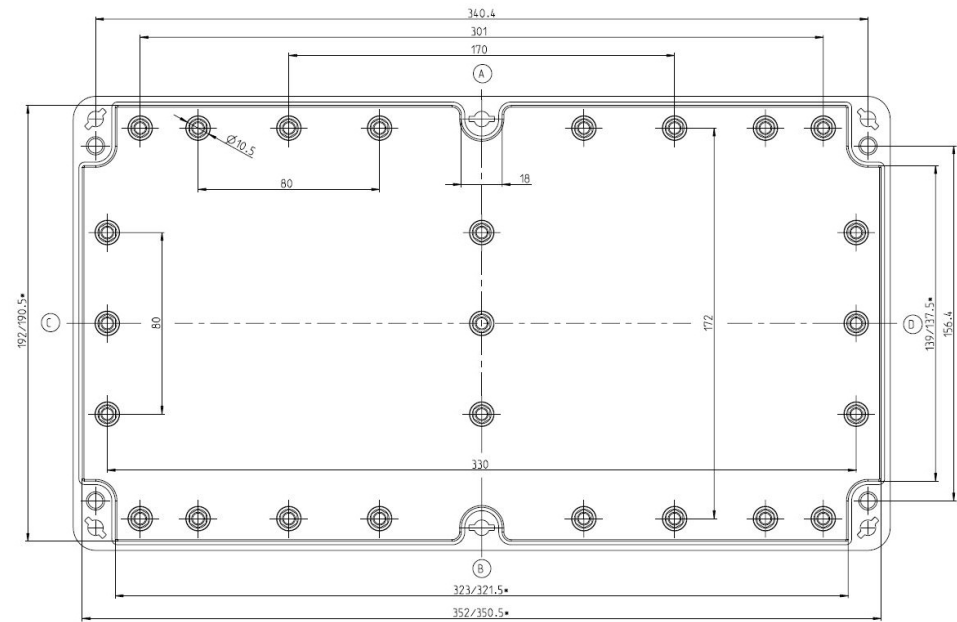
Base
