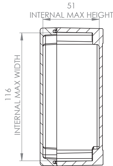
SECTION B-B
